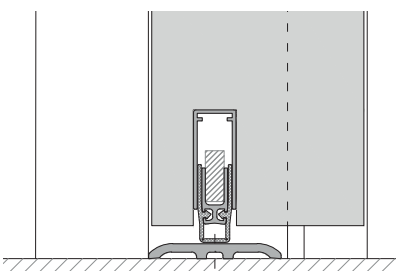
Door element ceiling and floor connection
