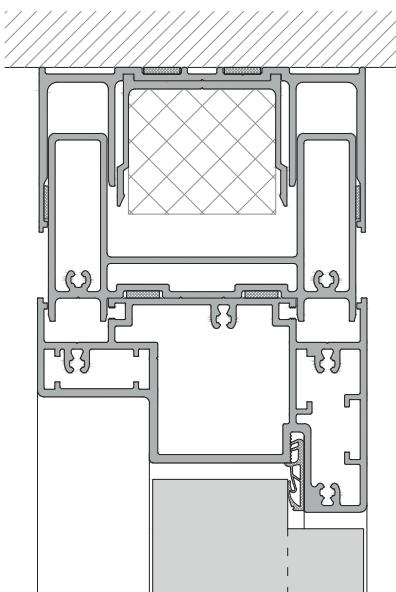
Glass element modular grid joint
