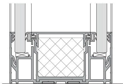
Glass element ceiling and floor connection
