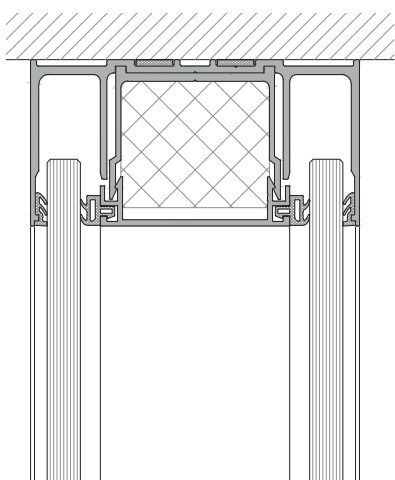
Glass element wall connection
